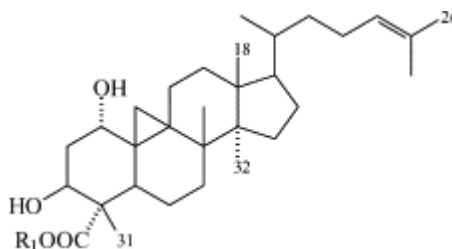
Molic acid and derivatives (Panzini et al. , 1993)
